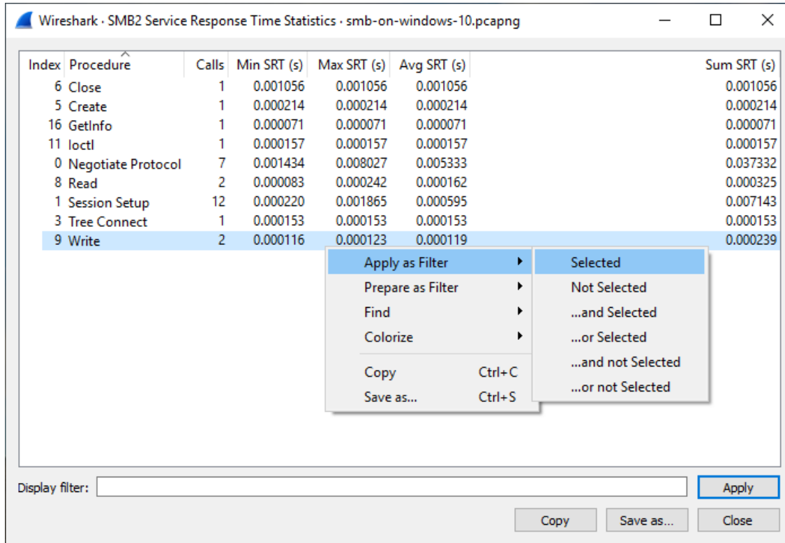
Figure 79. The “SMB2 Service Response Time Statistics” window
