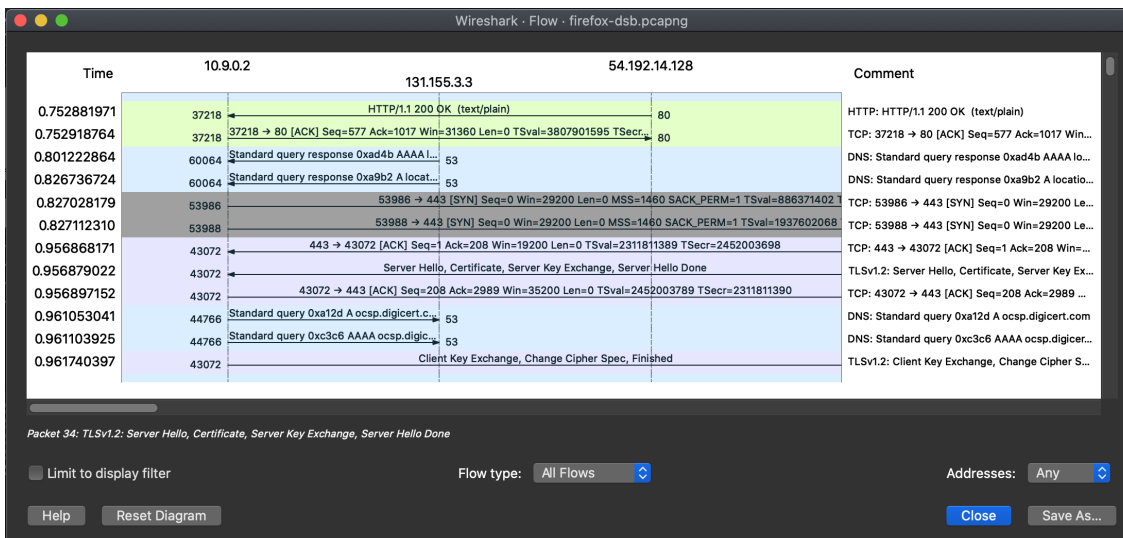
Figure 81. Flow Graph window
