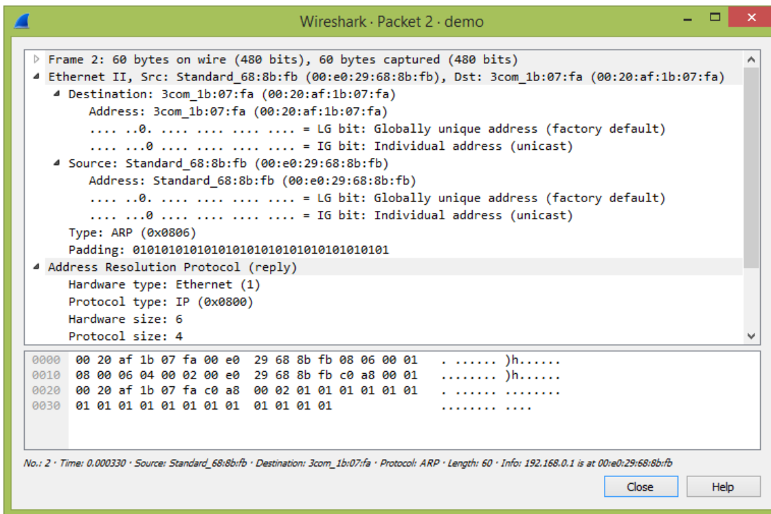
Figure 53. Viewing a packet in a separate window
