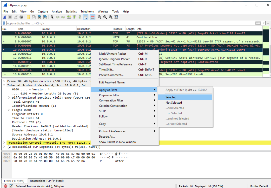
Figure 55. Pop-up menu of the “Packet List” pane
