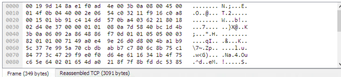
Figure 71. The “Packet Bytes” pane with a reassembled tab
