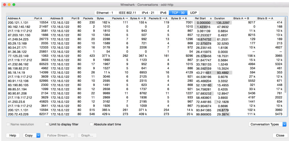
Figure 75. The “Conversations” window
