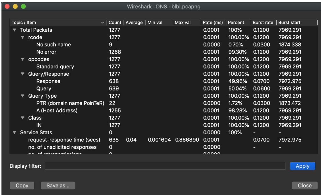
Figure 80. DNS statistics window
