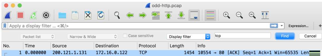
Figure 62. The “Find Packet” toolbar
