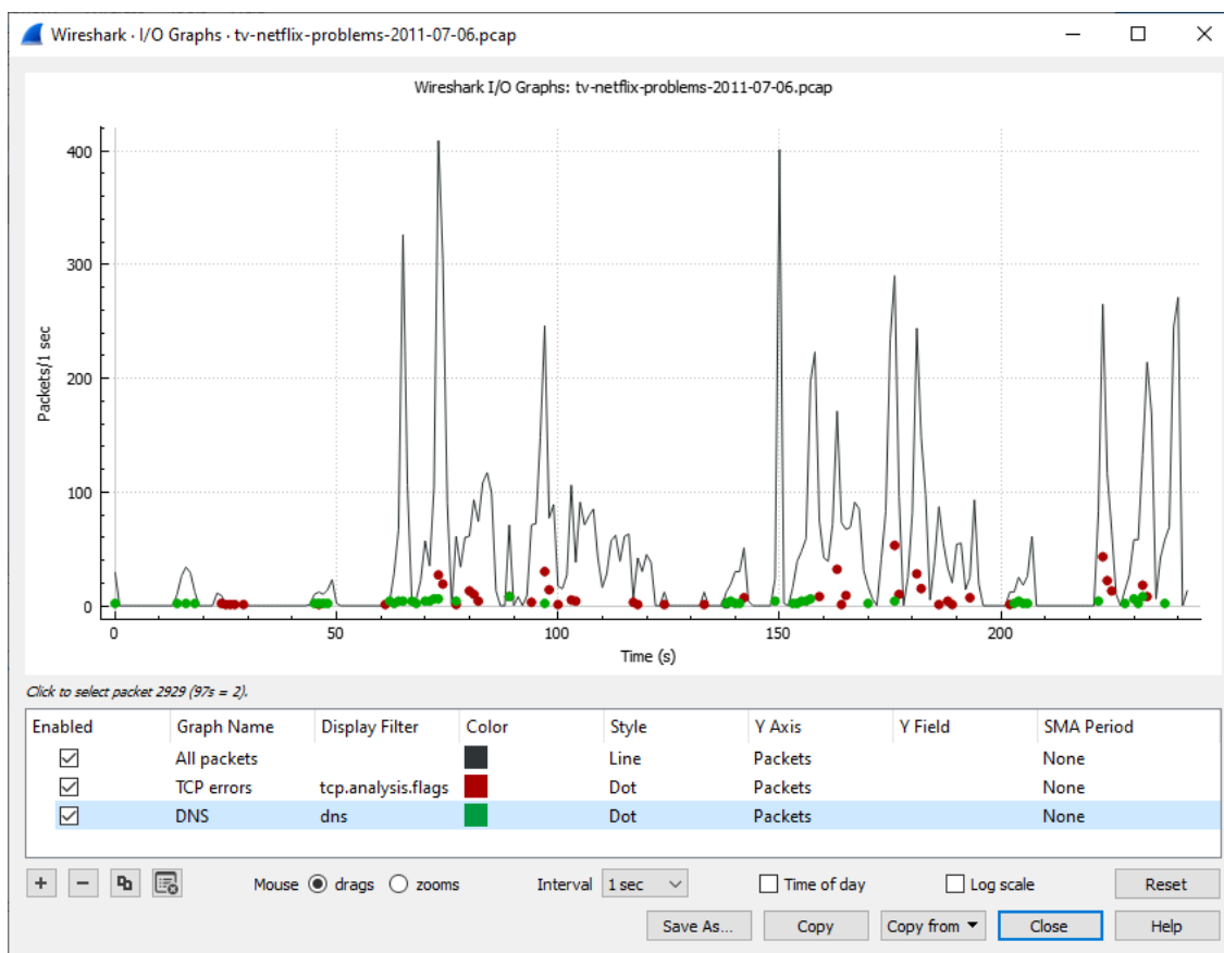
Figure 78. The “I/O Graphs” window
