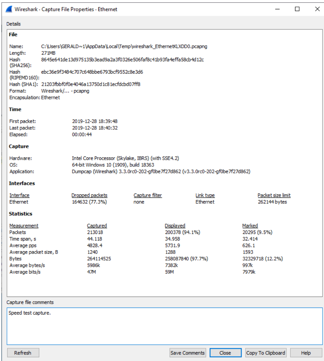
Figure 72. The “Capture File Properties” dialog
