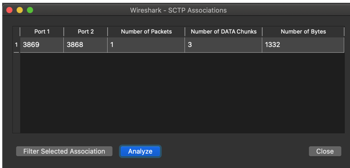
Figure 89. Sctp Associations window
