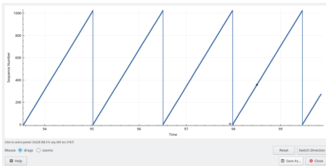
Figure 85. The RLC Graph window
