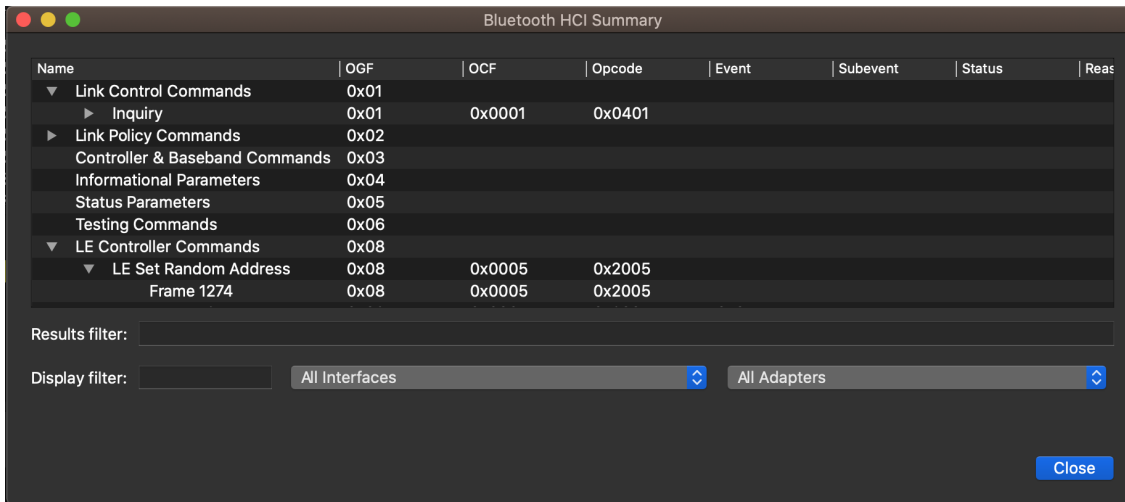
Figure 91. Bluetooth HCI Summary window
