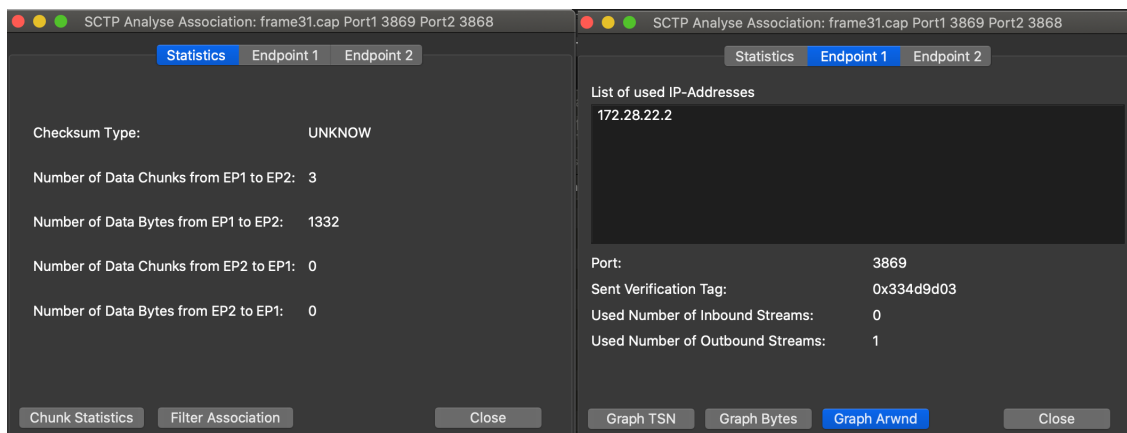
Figure 88. Sctp Analyze Association window
