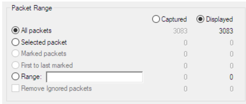
Figure 50. The “Packet Range” frame
