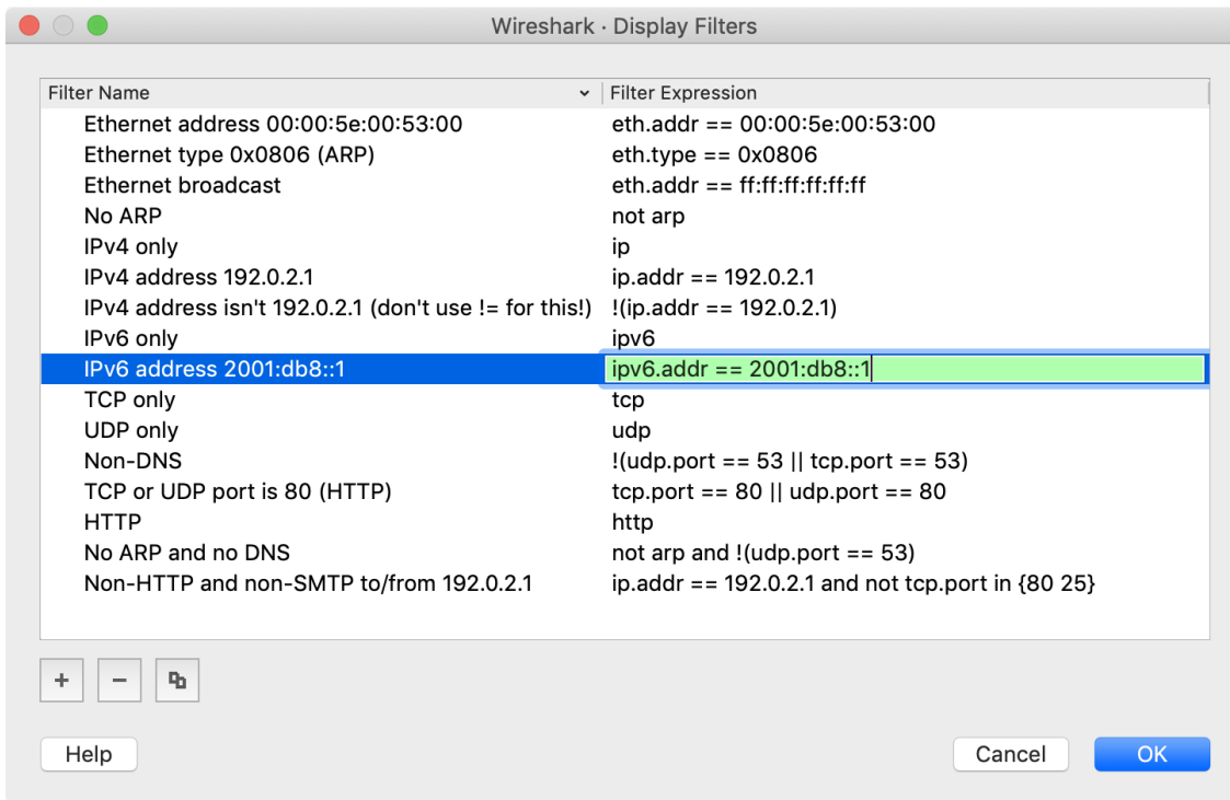
Figure 60. The “Capture Filters” and “Display Filters” dialog boxes
