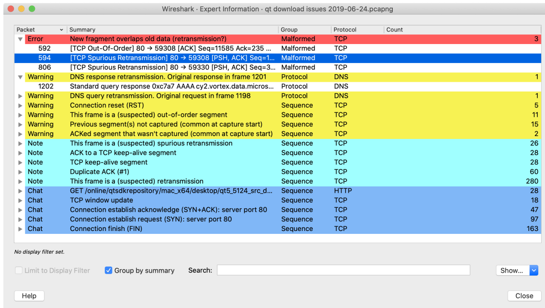
Figure 67. The “Expert Information” dialog box
