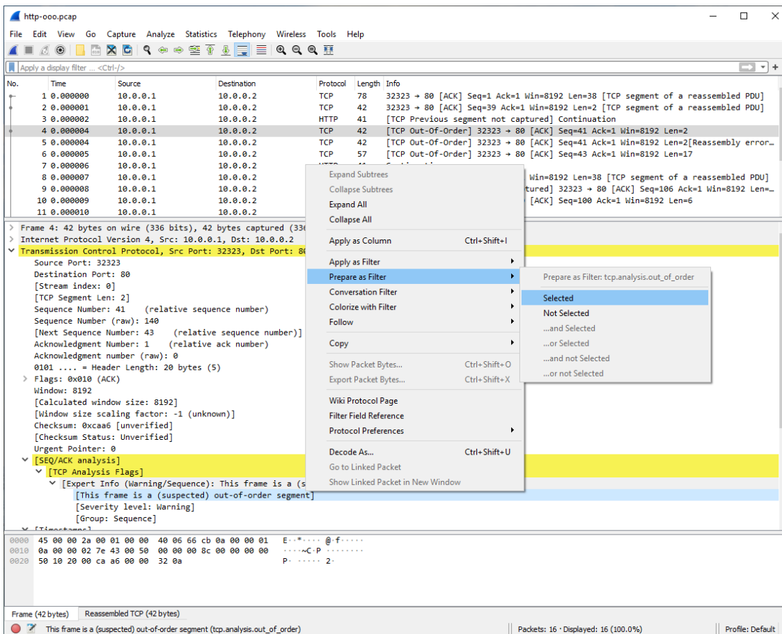
Figure 56. Pop-up menu of the “Packet Details” pane
