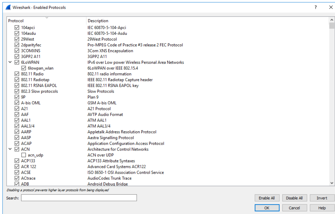
Figure 96. The “Enabled Protocols” dialog box
